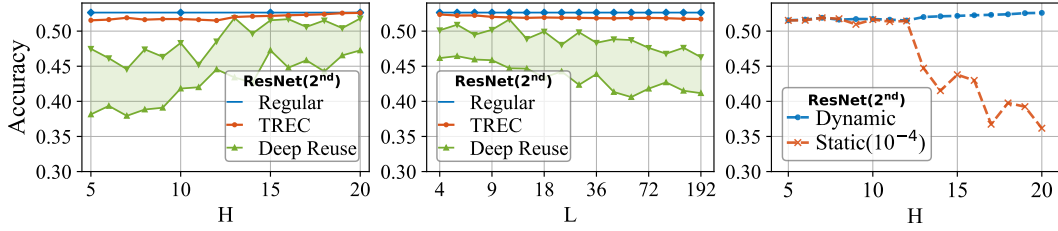
Figure 9: Effects of LSH parameter configuration and dynamic/static \sigma on accuracy of ResNet-34.
